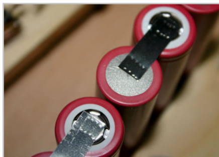
Laser Spot welding
